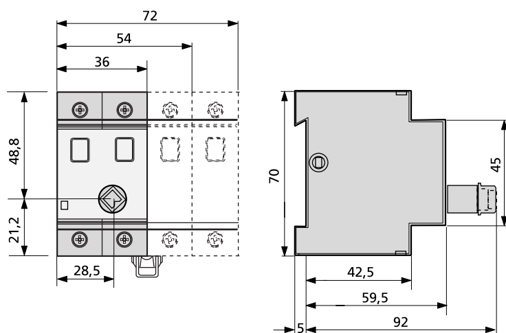
Duco, type DMV 40 - DMV 63, without knob.
