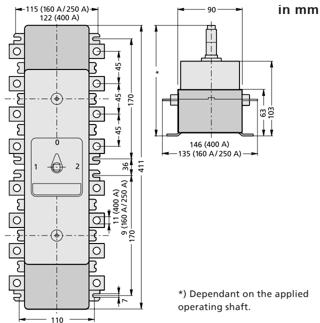
Change-over switches, Dumeco, Types DMVS 160N, DMV 250N and DMV 400N.
